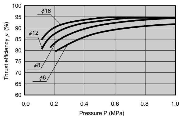
Fig. 2 Relations between thrust efficiency and pressure
