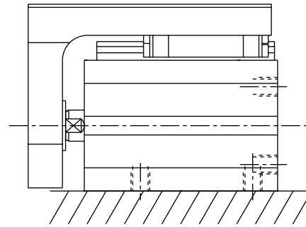
Side installation
