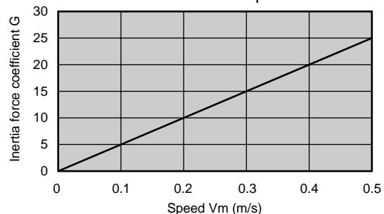
Fig. 1 Relations between inertia force coefficient and speed
